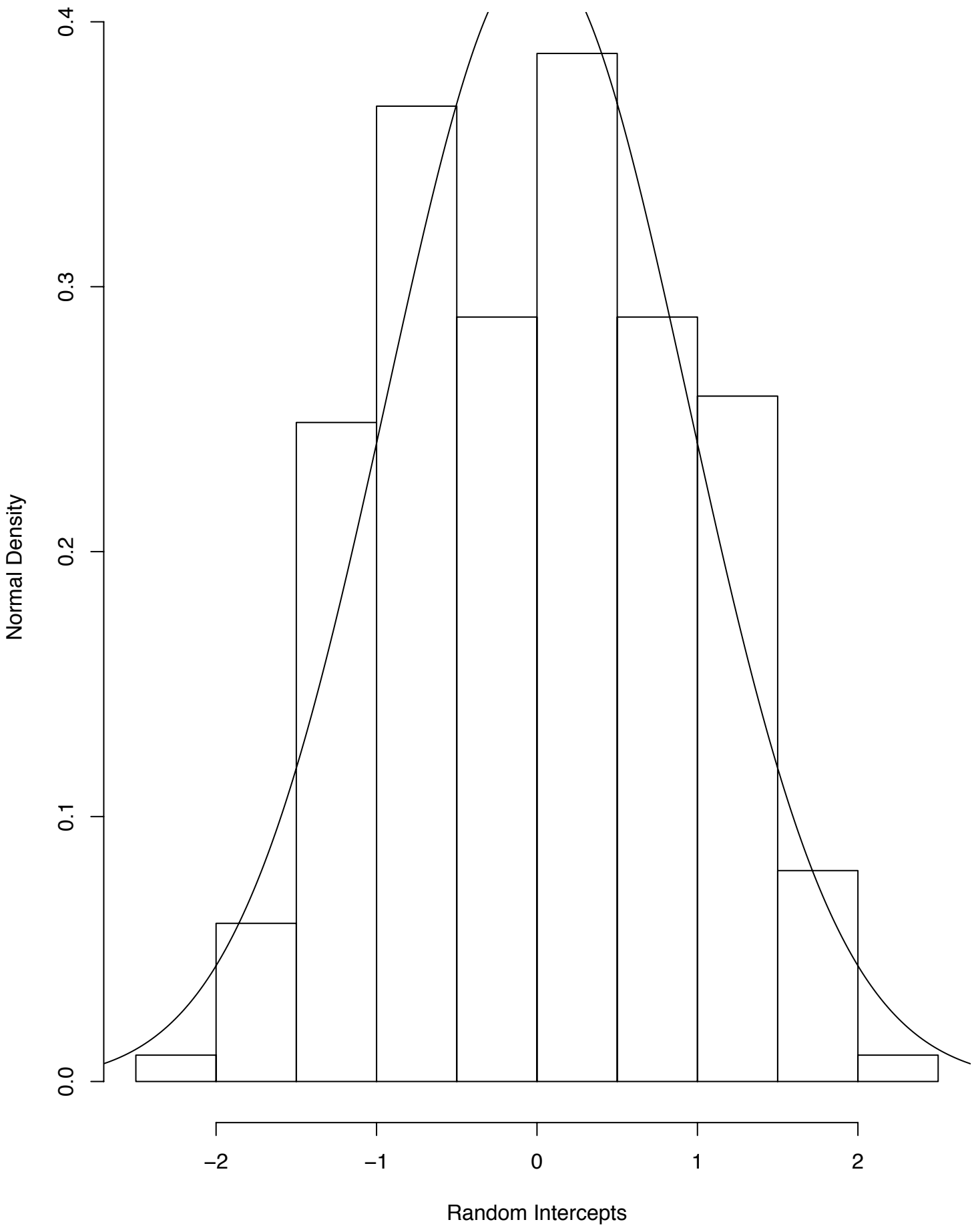
Histogram of Random Intercepts
